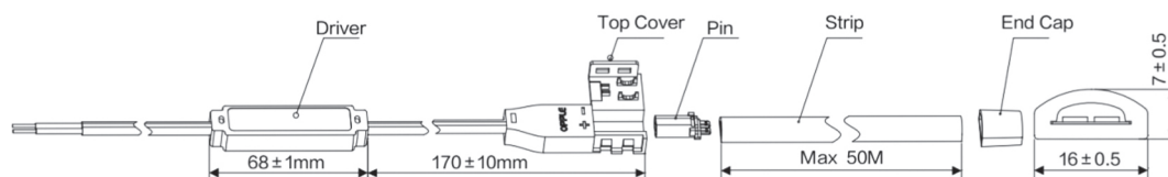
LED U Strip 2835 9W 120P
