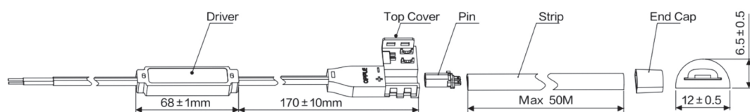
LED U Strip 2835 6W 60P
